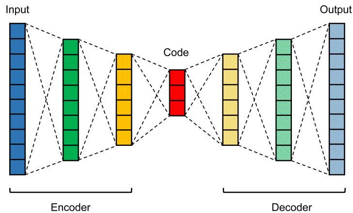
Figure 2.15: Basic structure of an Autoencoder.
