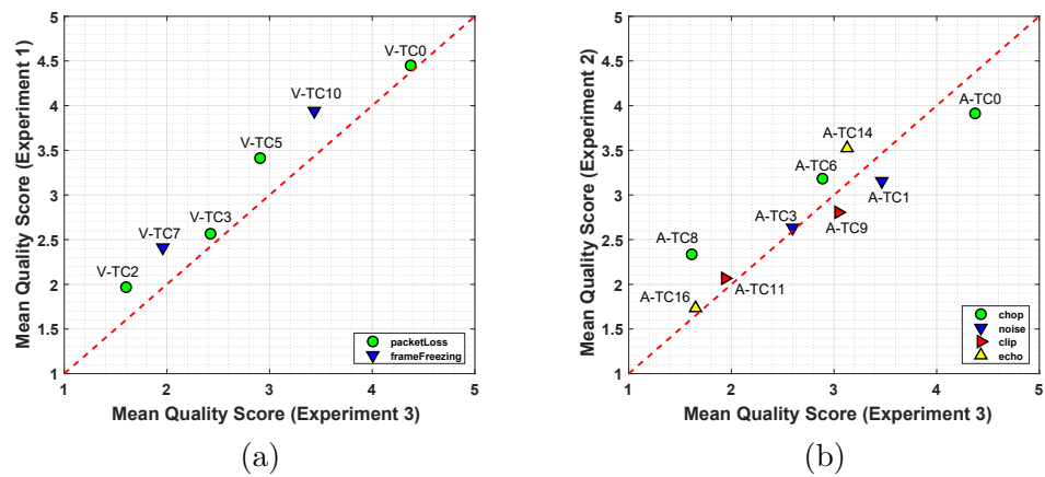
Figure 4.26: MQS results from experiment 1 and 3.
