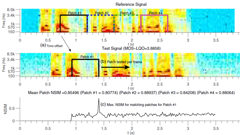
Figure 3.4: Visqol patch alignment and NSIM similarity. Original illustration from [115].
