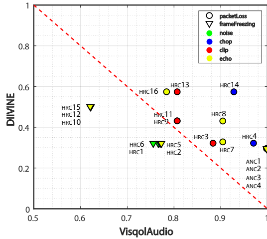
Figure 4.22: Scatter plot of audio objective scores (prduced by VISQOLAUDIO) versus video objective scores (produced by DIIVINE).
