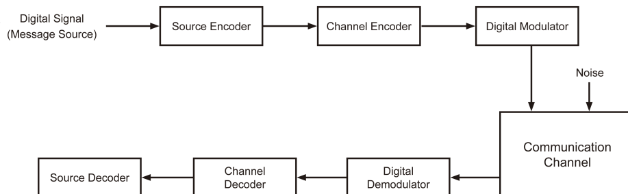
Figure 2.6: Basic diagram block of a digital communication system.
