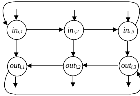
Figure 28.11 A clause gadget in the reduction from 3-SAT to DIRECTED-HAMILTONIAN-CIRCUIT
