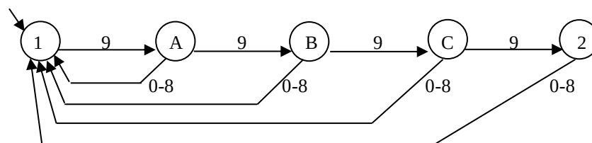
Figure 41.2 The code-entering fragment of a security system
