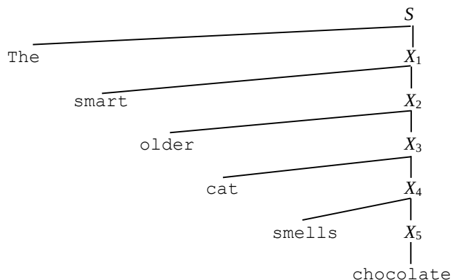
Figure 43.3 A parse tree that loses semantically meaningful structure
