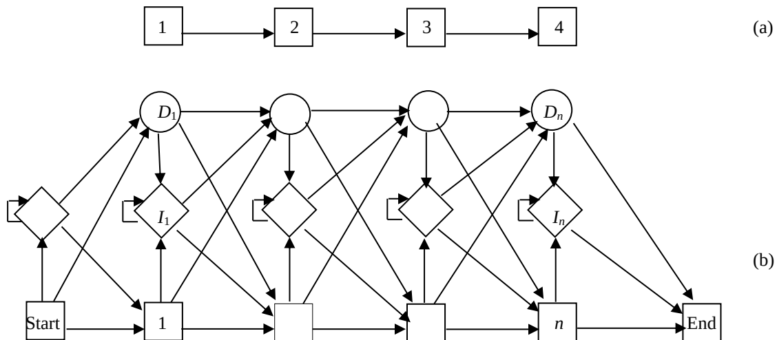
Figure 42.4 An HMM that describes a protein sequence family
