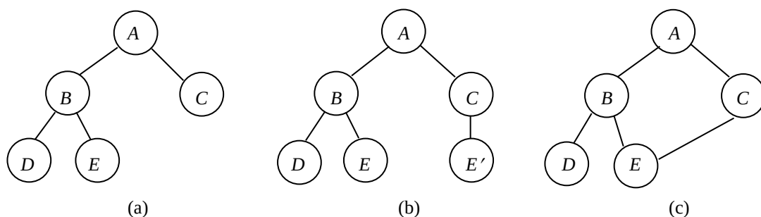
Figure 30.1 Tree search versus graph search
