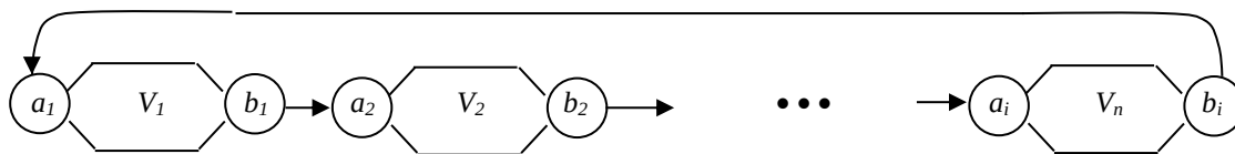
Figure 28.10 Stringing the variable gadgets together
