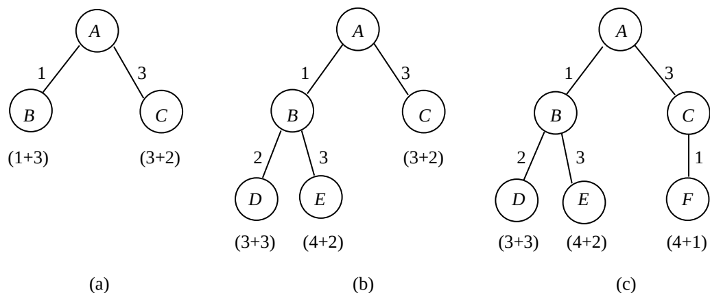
Figure 30.2 Best-first search
