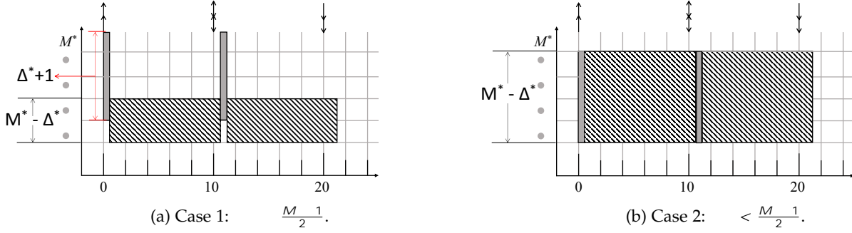
Fig. 6: For any M and \lambda_{\max} , there exists an SRT-infeasible system with total utilization greater than but arbitrarily close to (M - \lambda_{\max}) .
