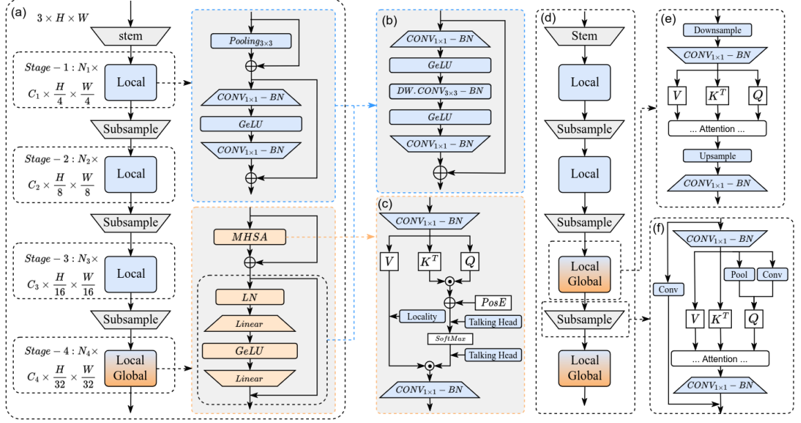
Figure 2.11. EfficientFormerV2 architecture with local and global processing blocks across four stages, unified FFN design, MHSA enhancements, and dual-path attention downsampling. Source: Rethinking Vision Transformers for MobileNet Size and Speed (LI et al. , 2022b)
