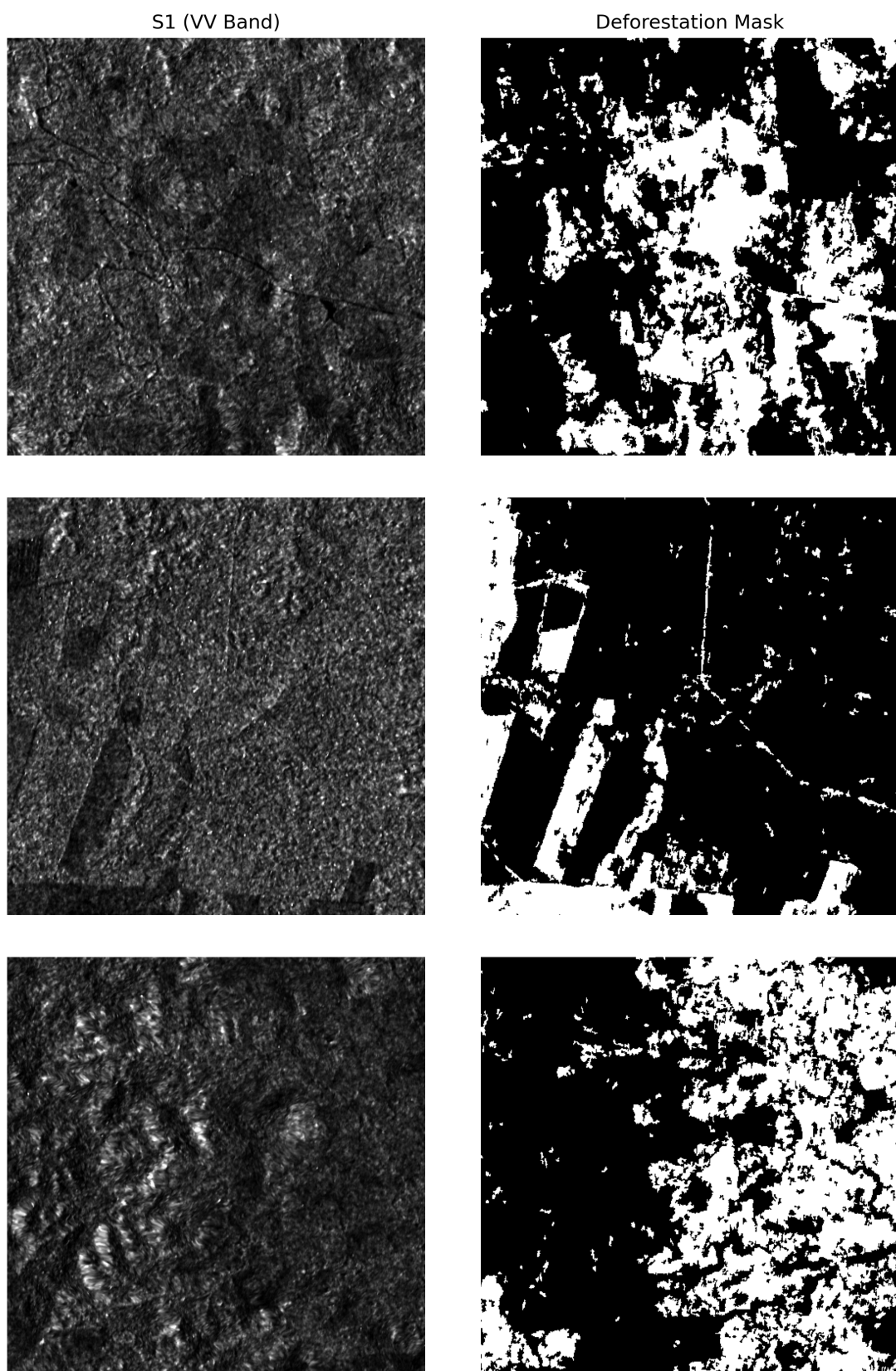
Figure 2.5. Crops from captures of the processed VV band Sentinel 1 next to the corresponding mask obtained by the described process.
