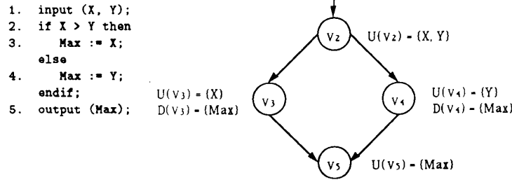
Fig. 1. Max program and its def/use graph.
