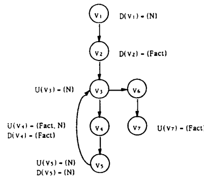
Fig. 2. Factorial program and its def/use graph.
